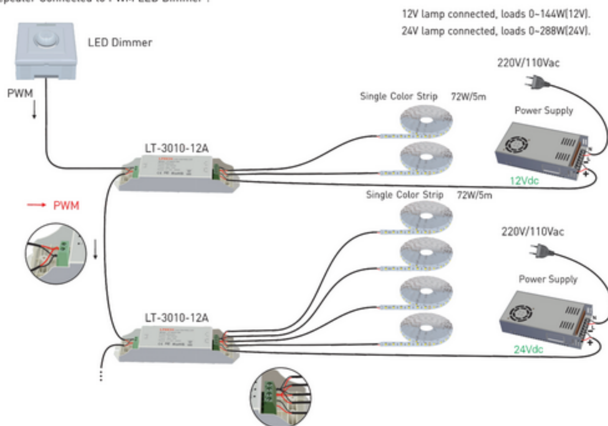
Power Repeater Connected to PWM LED Dimmer :
