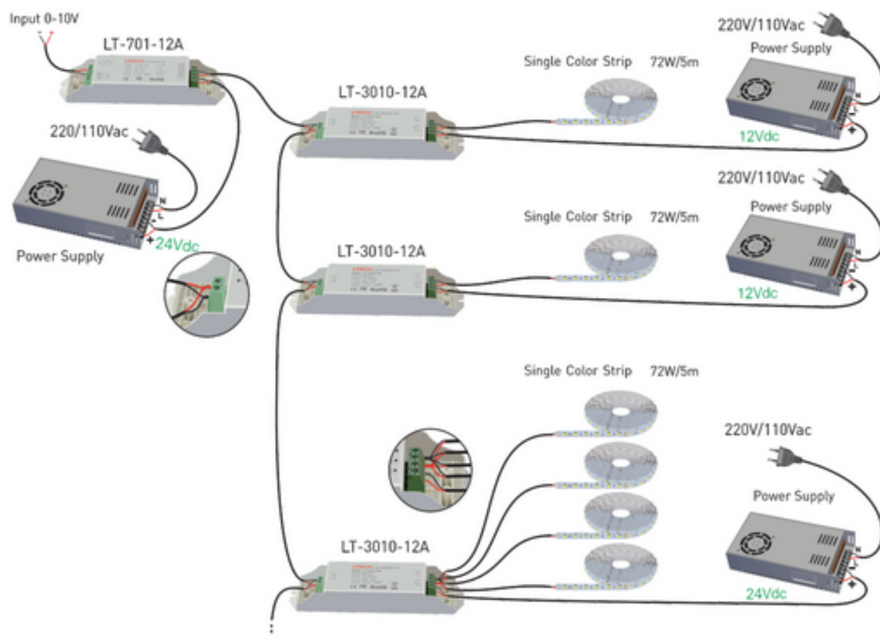
Power Repeater Connected to LED Dimmer:
