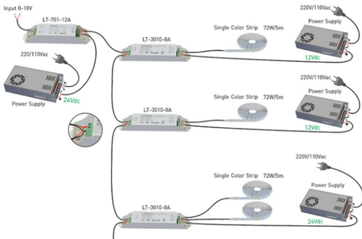
Power repeater connected to LED dimming driver:
