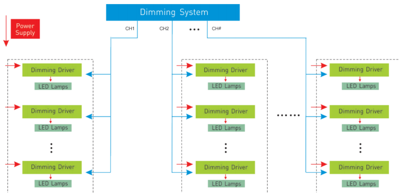
System Connection Diagram:
